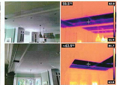
Radiant Cooling thermal image
